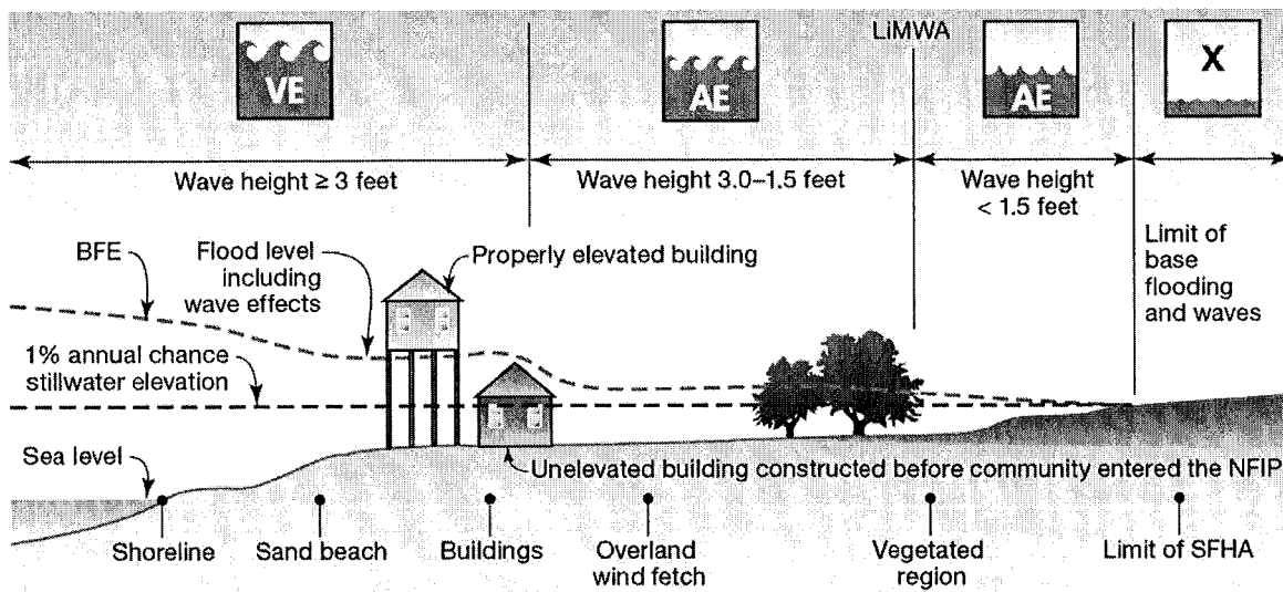
FIGURE 1 – TRANSECT SCHEMATIC
