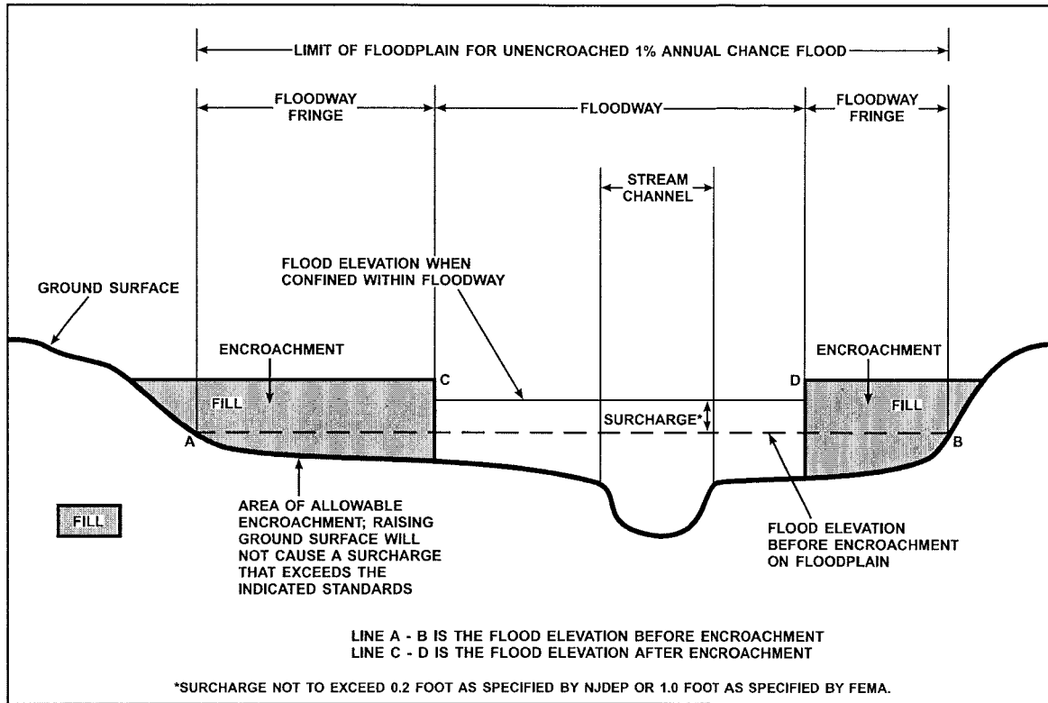
FIGURE 3 – FLOODWAY SCHEMATIC
